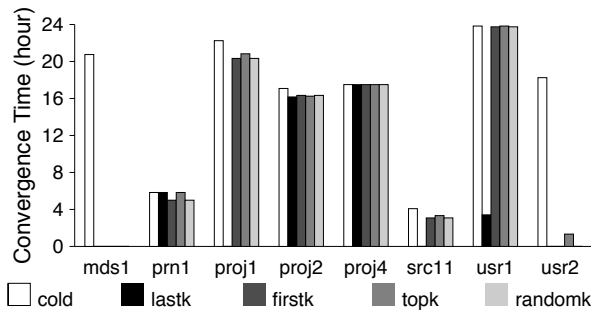
Figure 6: Convergence Time
